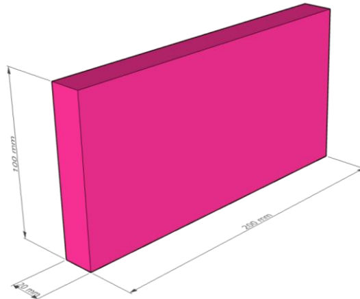
Figure 13: Dimensions of the parking lot limitations
